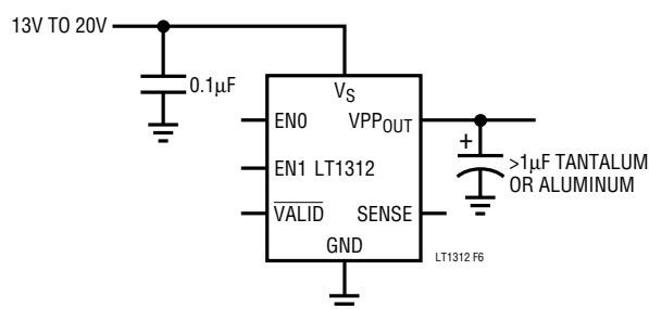
Figure 6. Recommended >1µF Tantalum Output Capacitor
