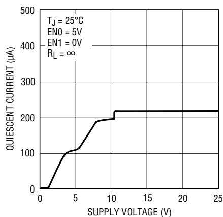
Quiescent Current (12V Mode)
